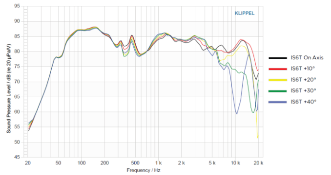
・垂直周波数応答 @1m(dB) 1 METER VERTICAL FREQUENCY RESPONSE
