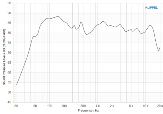
・軸上周波数応答 @1m(dB) 1 METER ON AXIS FREQUENCY RESPONSE
