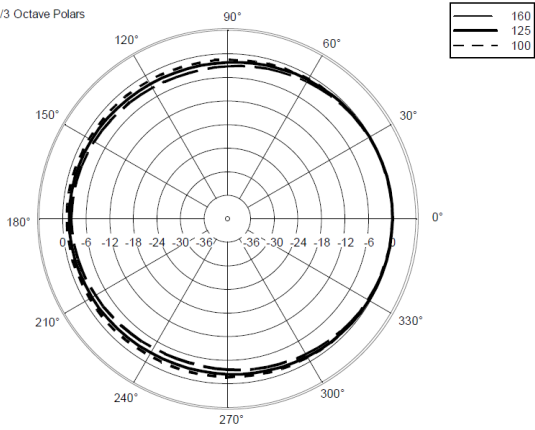
Vertical 1/3 Octave Polars
