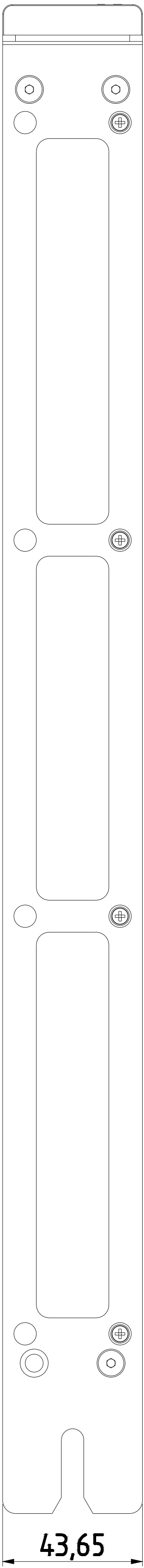
SIDE VIEW
