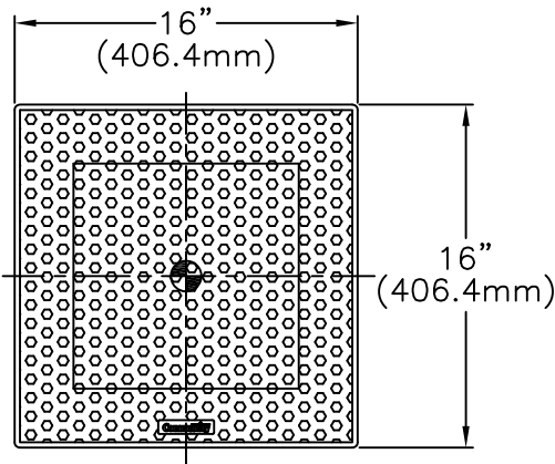
FRONT VIEW R-5HP
