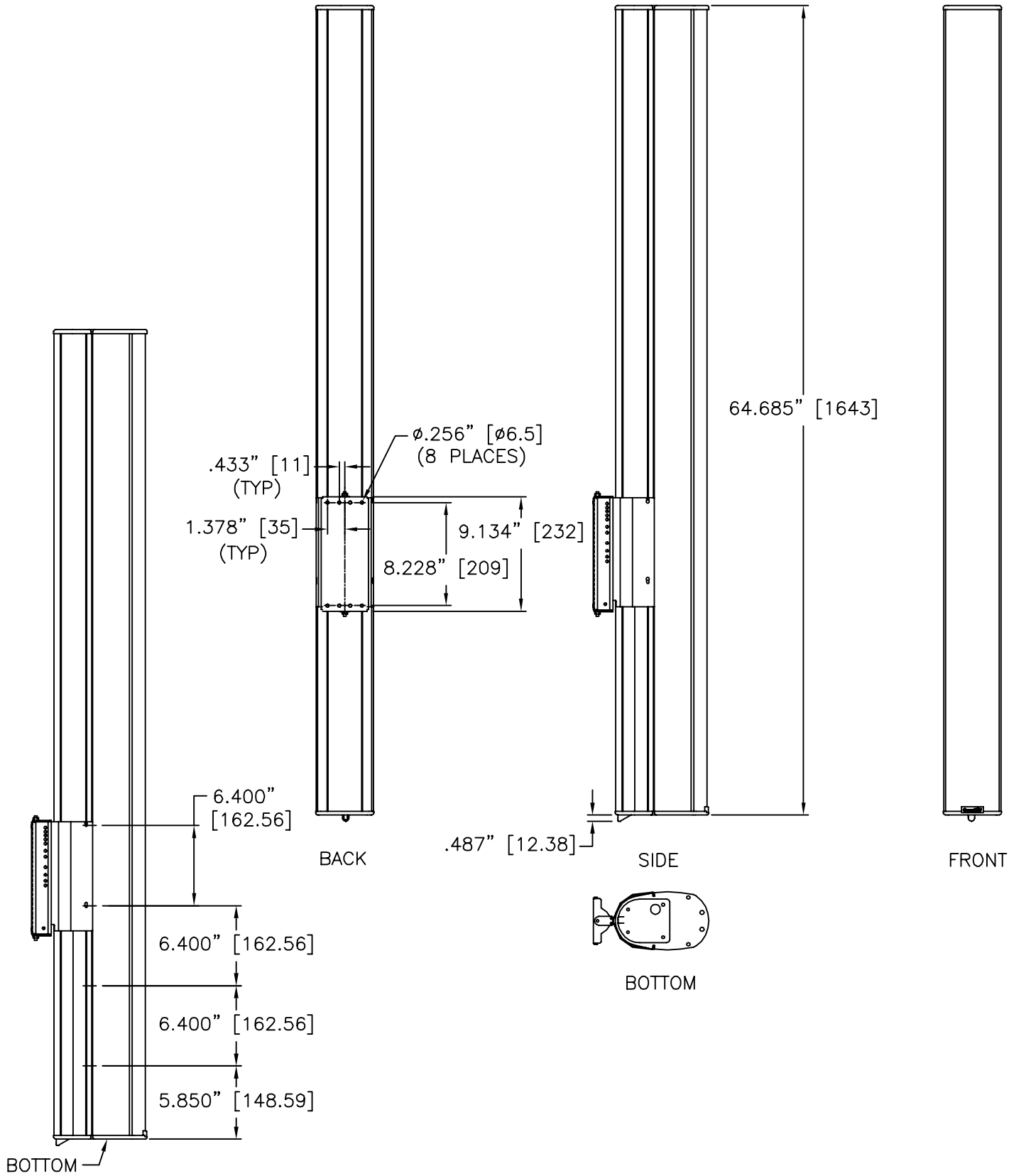
BRACKET ATTACHMENT HOLE LOCATIONS
